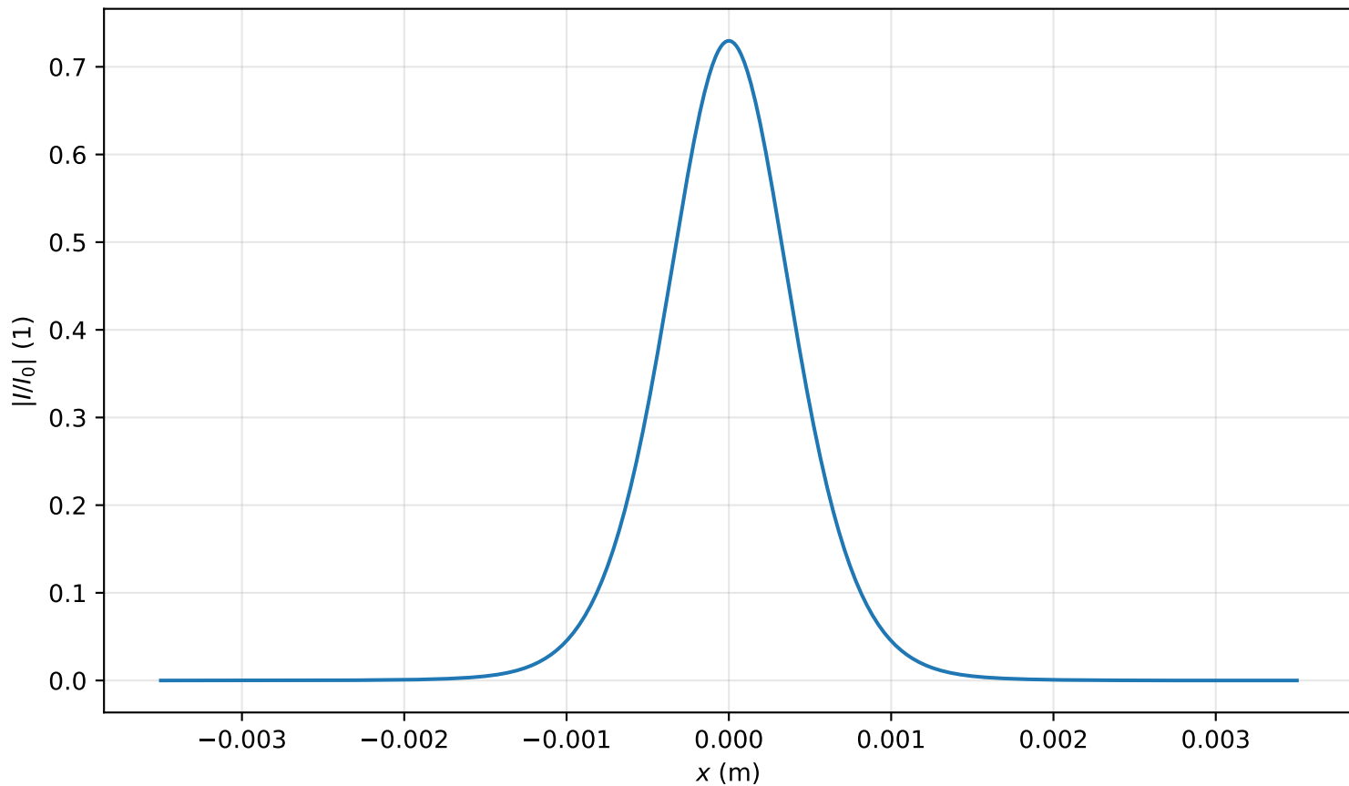
Intensity profile I(x, y = 0, z = 2.786m)/I_0 , P_{in}=0.6P_{cr} , artificial time
